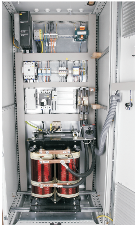
Compact assembly with thyristor and transformer
